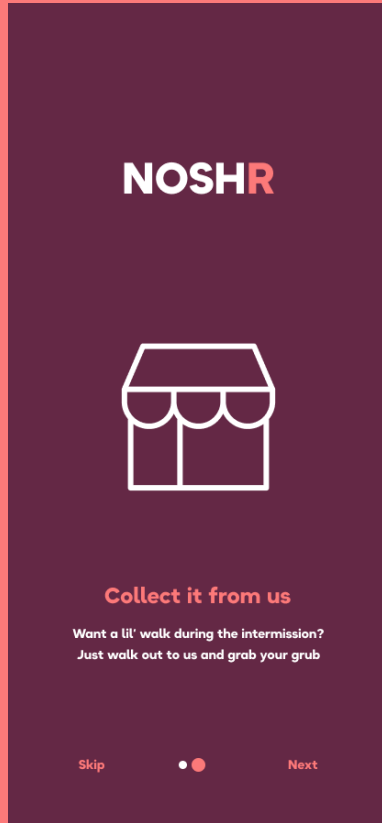
Onboarding Screens
